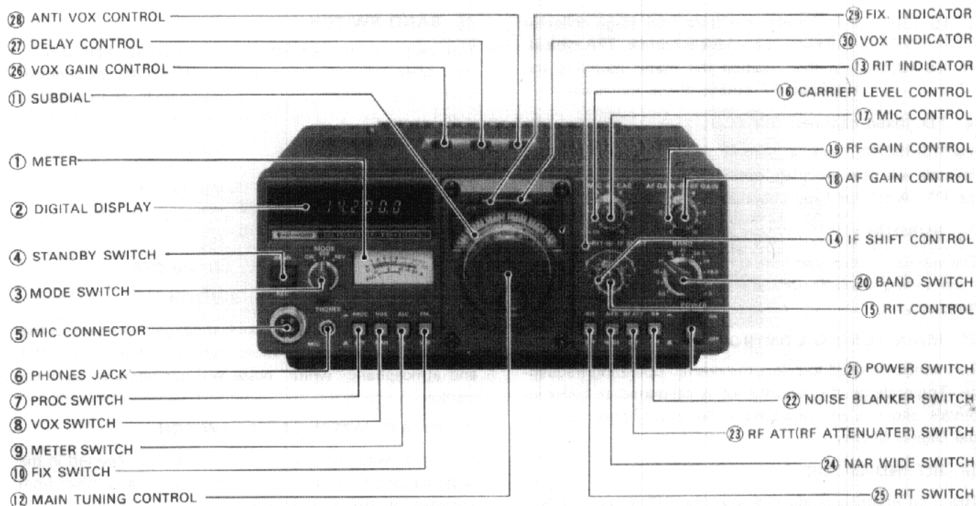
Fig. 3-1 Front Panel
