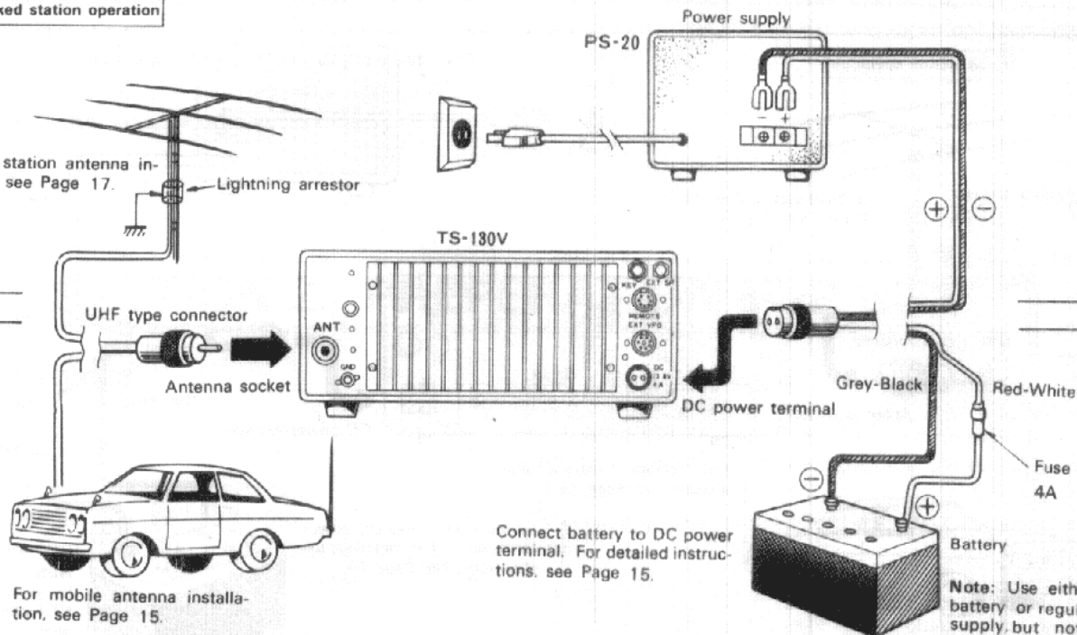
Fig. 2-2 [B] Antenna and Power Supply Connections of TS-130V
